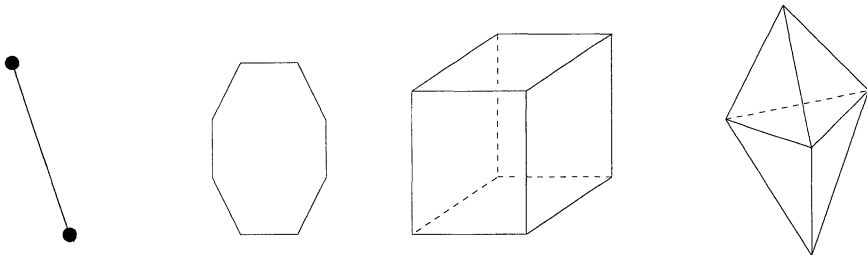
Figure 1.1. Polytopes in dimension one, two, and three
