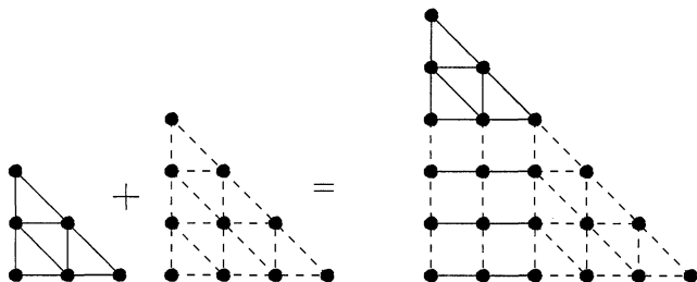
Figure 2.3. Mixed subdivision proving Bezout's Theorem
